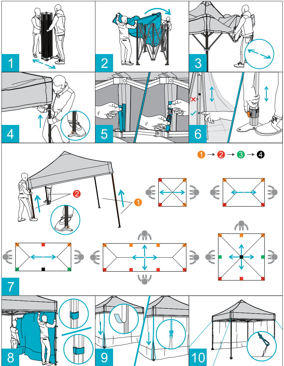
Fig. 2. Mounting process
